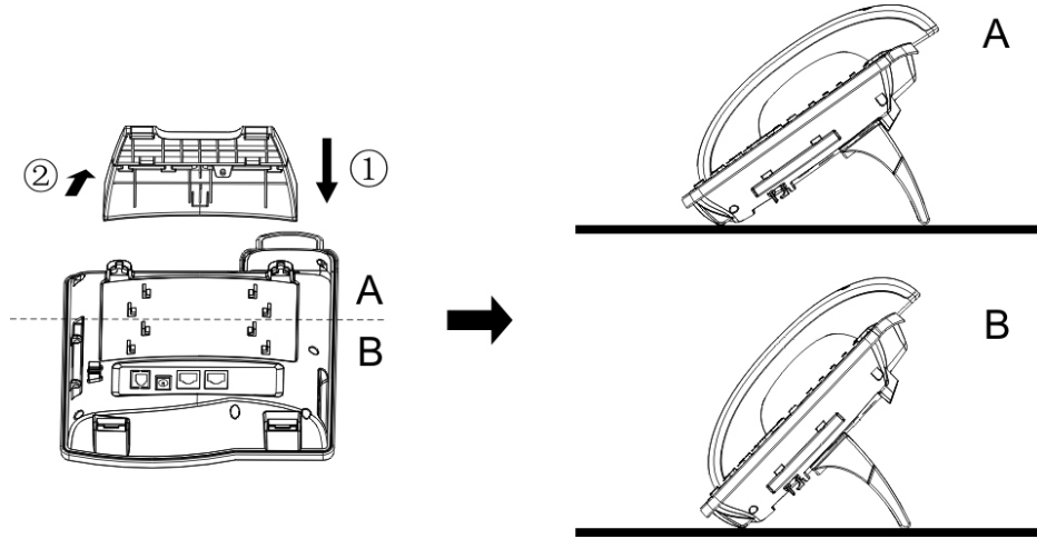
Figure 1 - Desktop Installation
