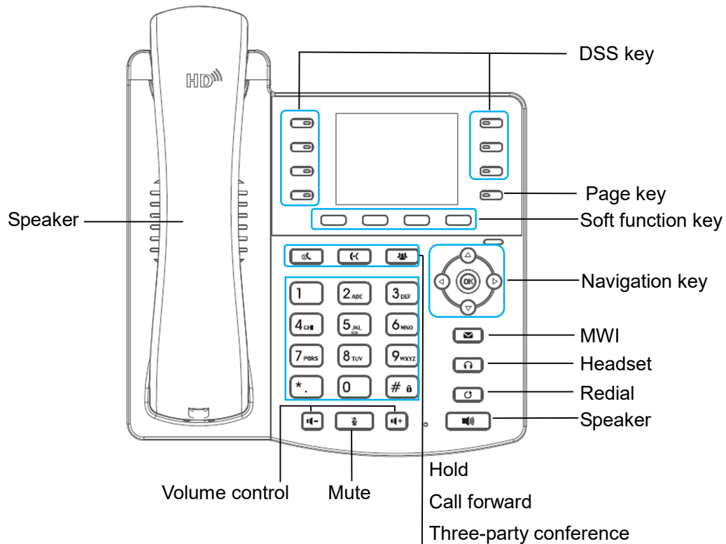
Figure 4 - Keypad
