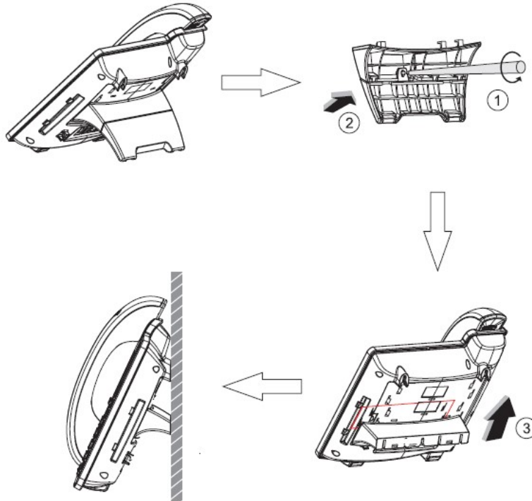
Figure 2 - Wall-mount Installation
